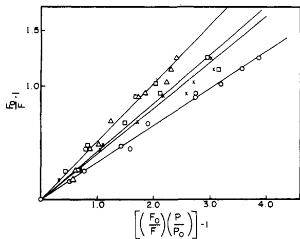
Figure 1. MBN xenon perturbation plots: 1 ( \Delta ), 2 ( \square ), 3 ( \times ), 4 ( \circ ).
