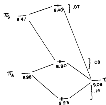
Figure 8. Orbital splitting diagram for MBN using corrected basis levels (see text).
