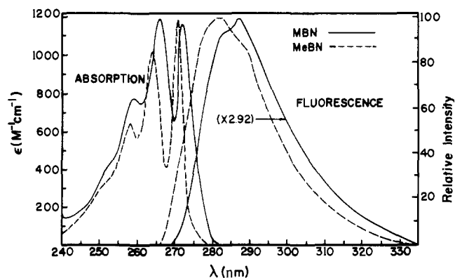
Figure 4. Absorption and fluorescence spectra for MBN and MeBN, in hexane at room temperature. (Note that the MBN fluorescence is scaled up by a factor of 2.92).
