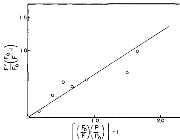
Figure 2. Xenon perturbation determination of \phi_{isc} for BN.
