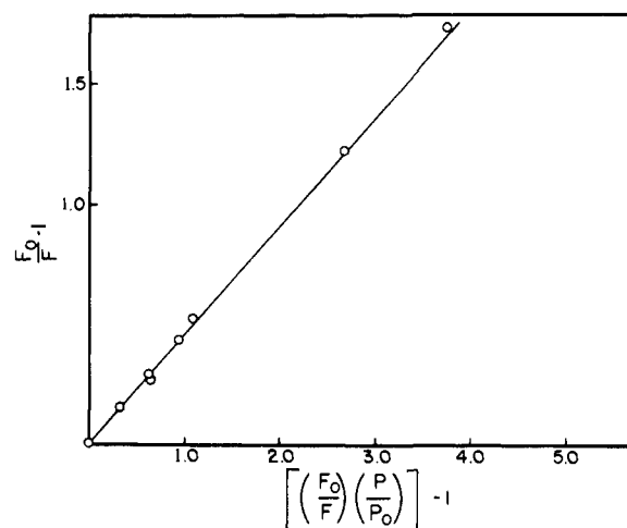
Figure 3. IBN xenon perturbation plot.
