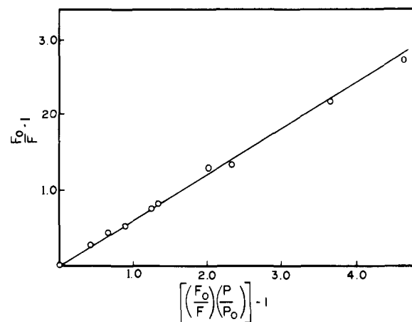
Figure 5. E -EMI xenon perturbation plot.
