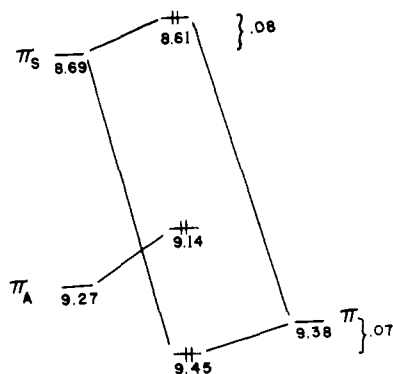
Figure 9. Orbital splitting diagram for 2-methyleneindan using corrected basis levels (see text).
