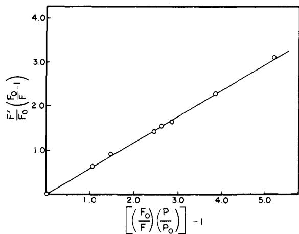
Figure 6. Xenon perturbation determination of \phi_{isc} for 1-methylindan.
