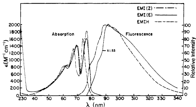
Figure 7. Absorption and fluorescence spectra for EMI and EMIH, in hexane at room temperature. (Note that the E -EMI fluorescence is scaled up by a factor of 1.53).
